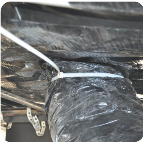
3. Secure vapor retarder layer at boots
